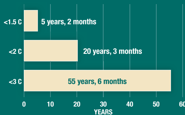
Estimated Number of Years Before Carbon Budgets Are Used Up for Different Levels of Warming
